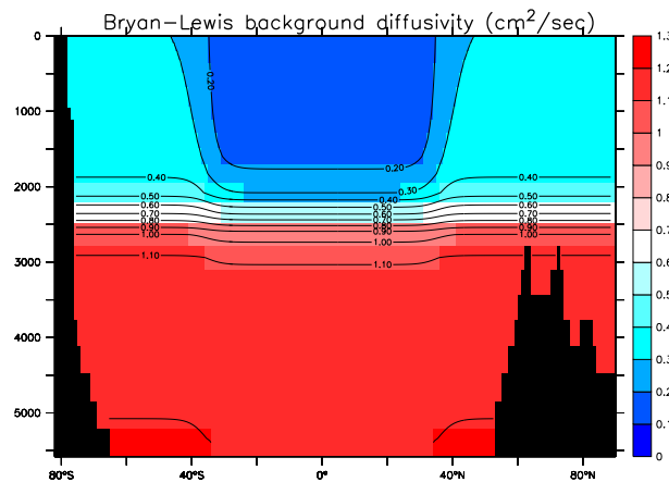
Figure 3.2: Shown here is the latitude dependent Bryan-Lewis diffusivity ( \text{cm}^2 \text{s}^{-1} ) based on values used in GFDL-CM2.1 configuration discussed in Griffies et al. (2005). The diffusivity is composed of the two profiles shown in Figure 3.1, with an exponential transition at 35^\circ from the lower values in the tropics to the larger values in the high latitudes.
