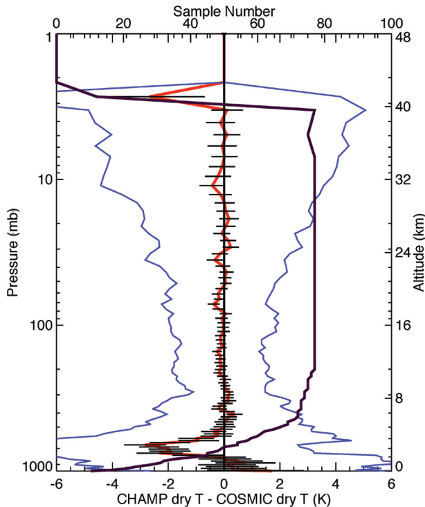
FIG. 14. Comparison statistics (mean: red; standard error of the mean: horizontal black lines superimposed on the mean; std dev: blue; sample number of compared soundings: solid black line) of 80 CHAMP and COSMIC profiles that were collocated within 200 km and 90 min from 1 Sep to 31 Oct 2006, within 60°S–60°N.
