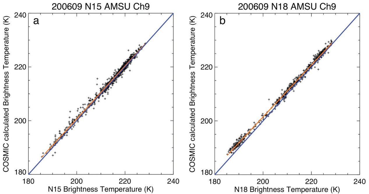
FIG. 16. Comparison of COSMIC-simulated AMSU Ch9 Tb and (a) NOAA-15 AMSU Ch9 Tb and (b) NOAA-18 AMSU Ch9 Tb for Sep 2006.
