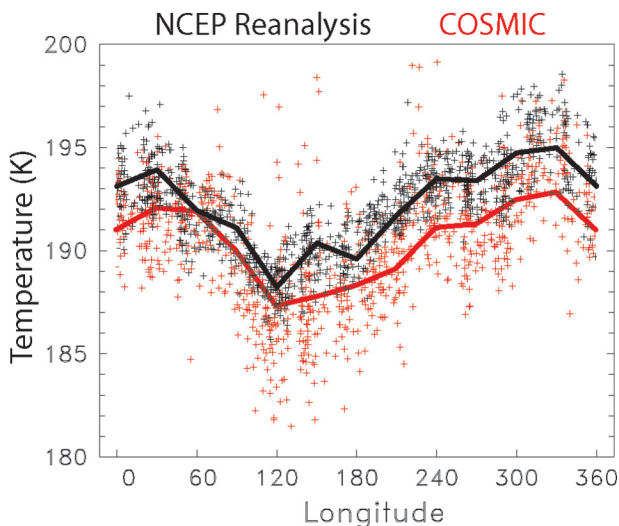
FIG. 17. Temperatures (red +) at the cold-point tropopause derived from all COSMIC temperature retrievals over 10^{\circ}\text{N} – 5^{\circ}\text{S} for 20–30 Dec 2006. Each point represents one sounding, and the red line indicates the average longitudinal structure. The black line denotes the cold-point tropopause average derived from NCEP reanalysis data for the same time period, with individual points (black +) sampled identically to the COSMIC data.
