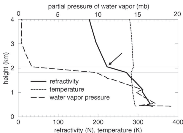
FIG. 4. Temperature, water vapor, and refractivity profiles in the lowest 4 km of the atmosphere, based on a radiosonde (2 Jan 2002; 15.97°S, 5.70°W) showing typical structure of the ABL (Sokolovskiy et al. 2006b).
