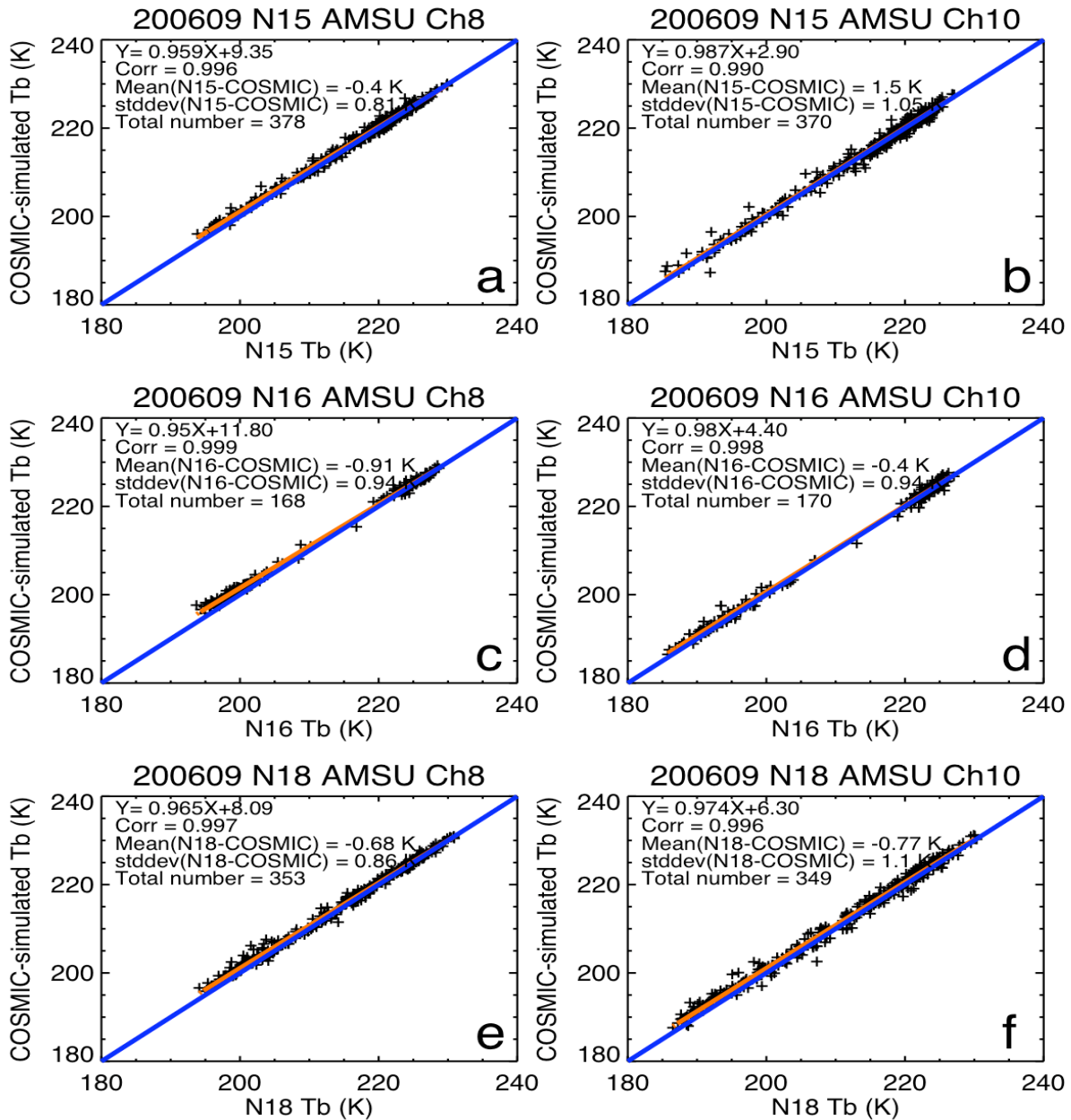
Figure 6: Comparison of (a) COSMIC-simulated AMSU Ch8 Tbs and NOAA 15 AMSU Ch8 Tbs, (b) COSMIC-simulated AMSU Ch10 Tbs and NOAA 15 AMSU Ch10 Tbs, (c) COSMIC-simulated AMSU Ch8 Tbs and NOAA 16 AMSU Ch8 Tbs, (d) COSMIC-simulated AMSU Ch10 Tbs and NOAA 16 AMSU Ch10 Tbs, (e) COSMIC-simulated AMSU Ch8 Tbs and NOAA 18 AMSU Ch8 Tbs, (f) COSMIC-simulated AMSU Ch10 Tbs and NOAA 18 AMSU Ch10 Tbs.
