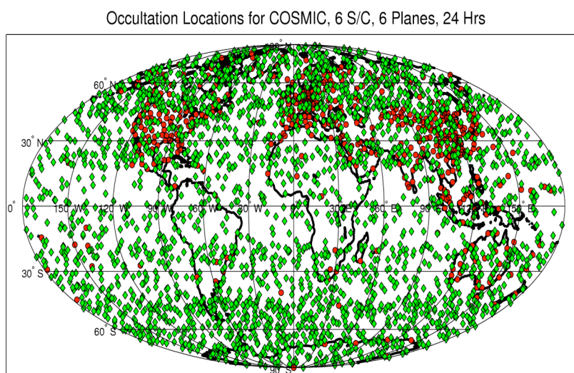
Figure 1: Typical operational distribution of COSMIC GPS radio occultation soundings (green dots) over a 24-h period over the globe. Red dots are locations of operational radiosonde stations.
