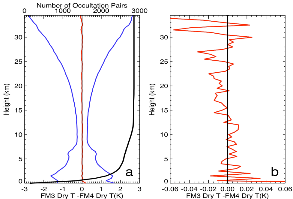
Figure 3: (a) The median and the median absolute deviation (MAD) of the dry temperature difference between two COSMIC satellites (FM3 and FM4) from 2006, day 111 through 300 where distance between FM3-FM4 receivers are within 10 km. The blue line is MAD to its median difference (in red) and the black line is number the FM3-FM4 profile pairs used in the comparison at various vertical levels, (b) median of the dry temperature difference between FM3-FM4 as (a) but in a much smaller temperature scale in x-axis.
