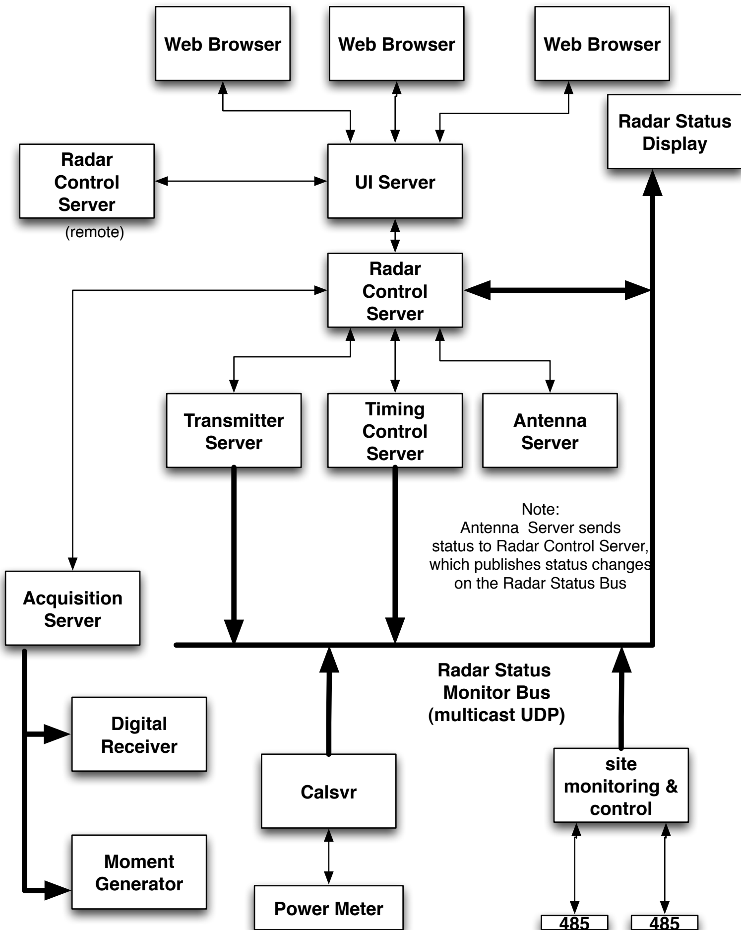
IWR System Control Architecture - revised 2009/11/9
