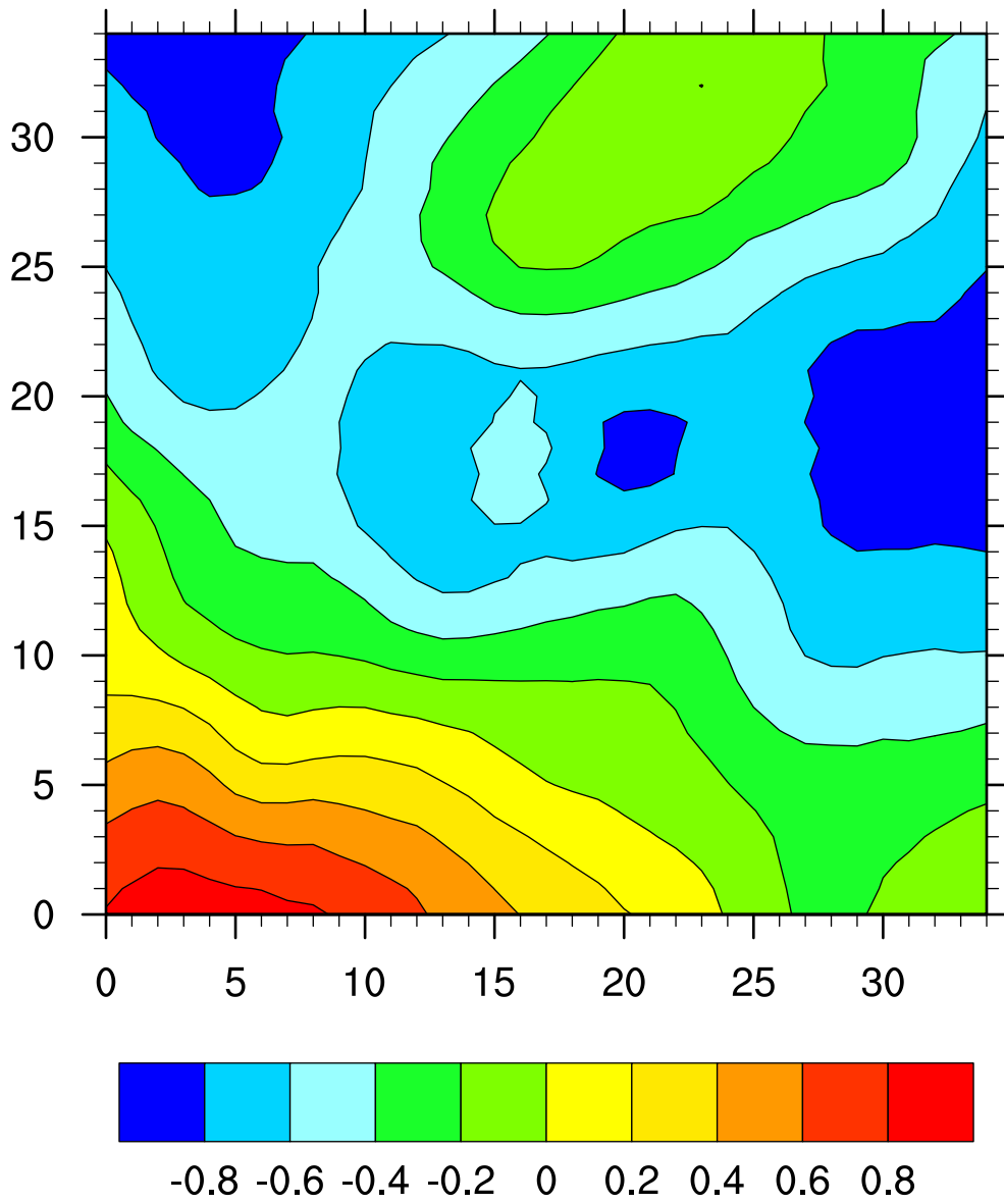
Negative MSLP bias evolution h54-60(hPa)
