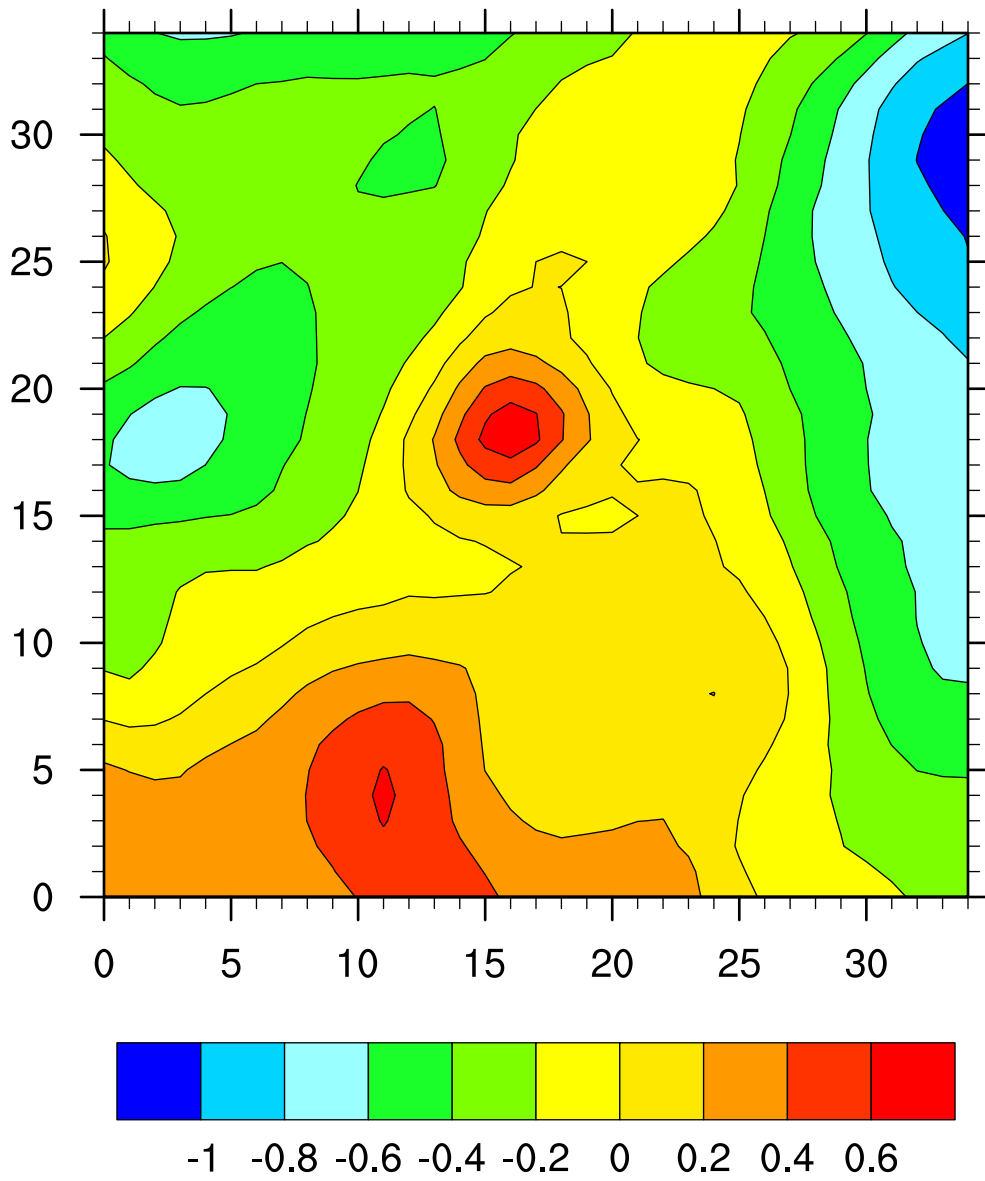
Negative MSLP bias evolution h30-36(hPa)
