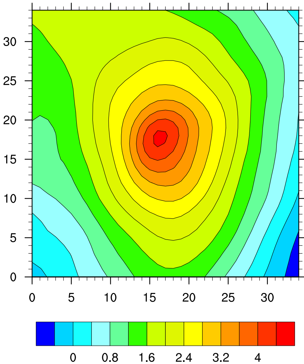
Positive MSLP bias evolution h78-84(hPa)
