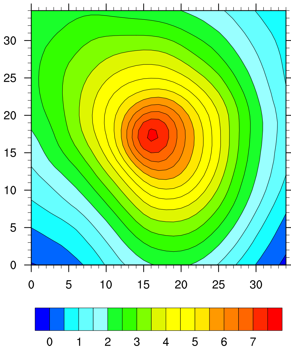
Positive MSLP bias evolution h90-96(hPa)
