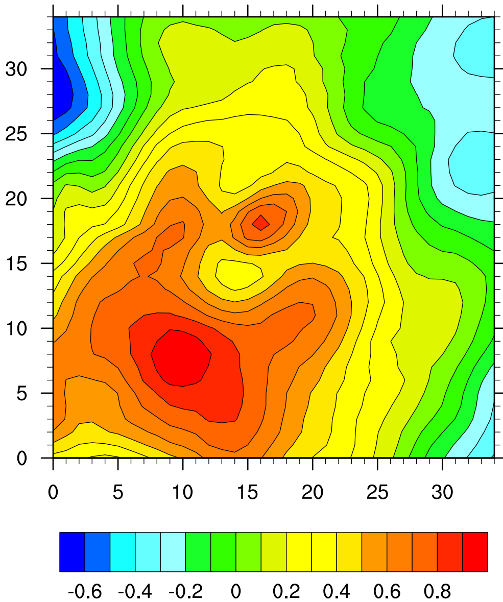
Positive MSLP bias evolution h30-36(hPa)
