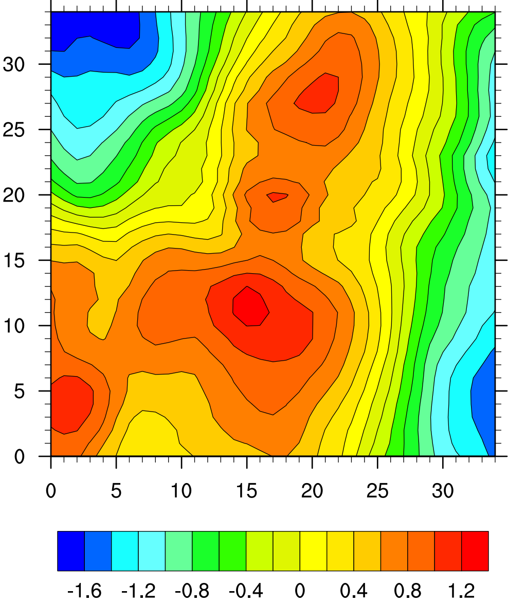
Positive MSLP bias evolution h6-12(hPa)
