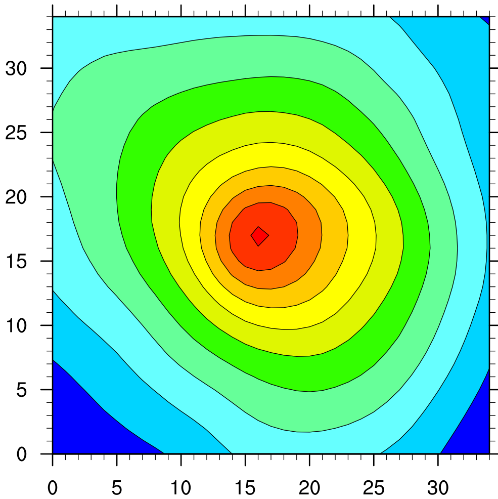
Positive MSLP bias evolution h102-108(hPa)
