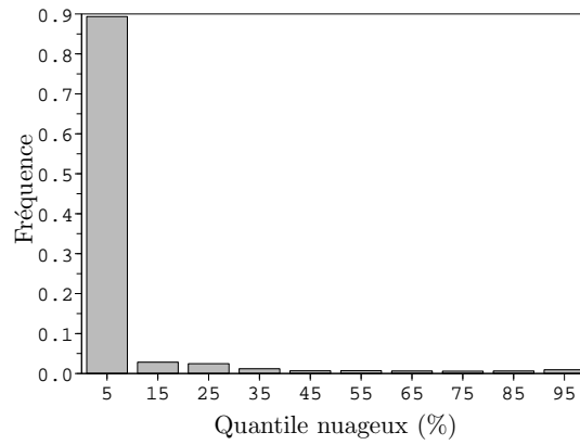
(b) Intrusions sèches, T_{\text{cld}} = -54 \text{ }^\circ\text{C}
