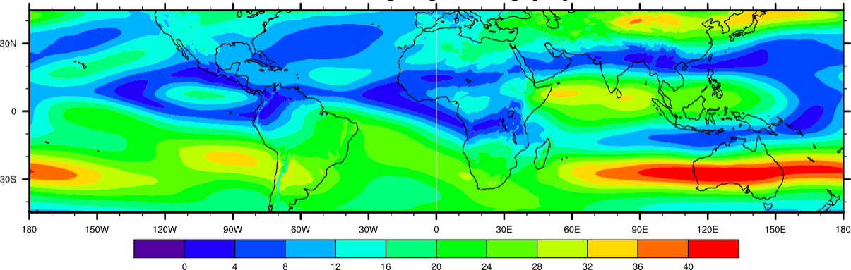
dudz Average Aug-Oct average [m/s]
