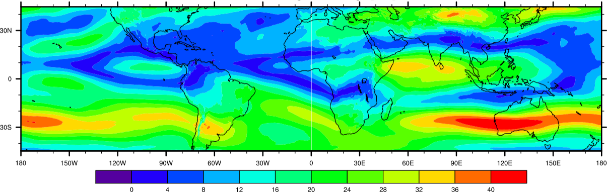
dudz 2005 Aug-Oct average [m/s]
