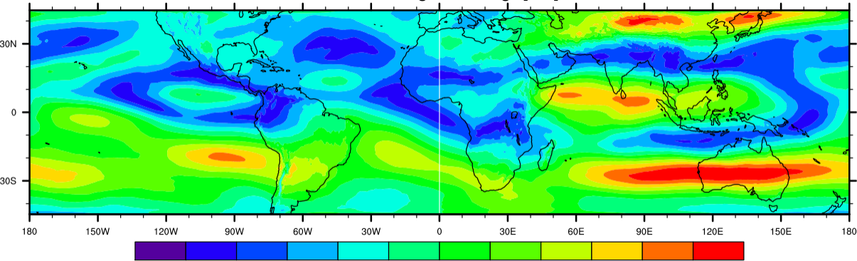
dudz 2001 Aug-Oct average [m/s]
