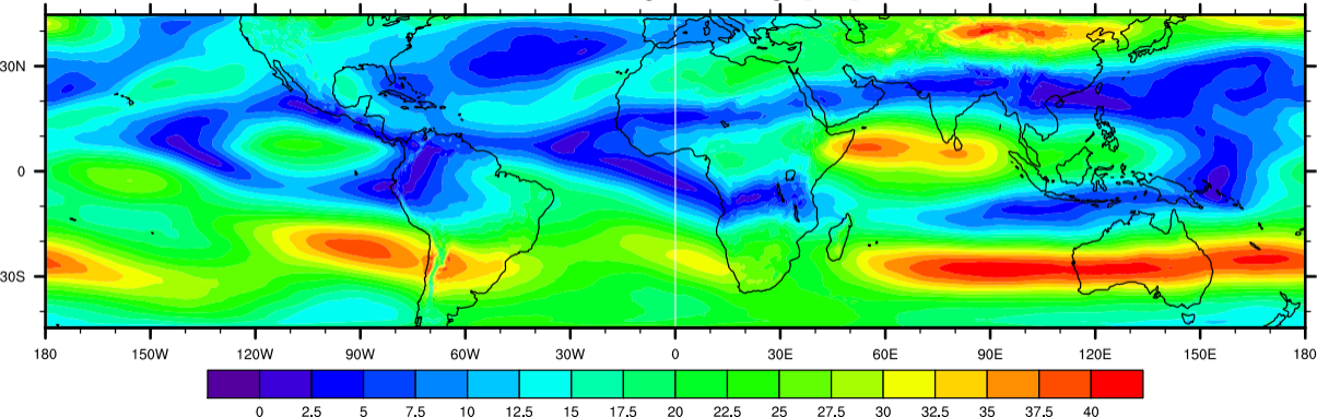
dudz 2000 Aug-Oct average [m/s]
