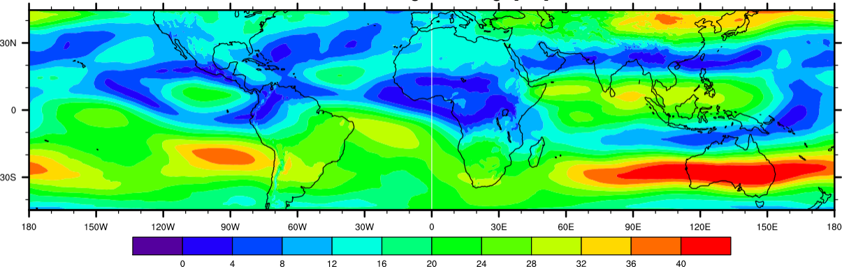
dudz 2003 Aug-Oct average [m/s]
