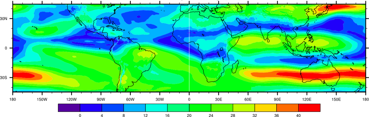
dudz 2002 Aug-Oct average [m/s]
