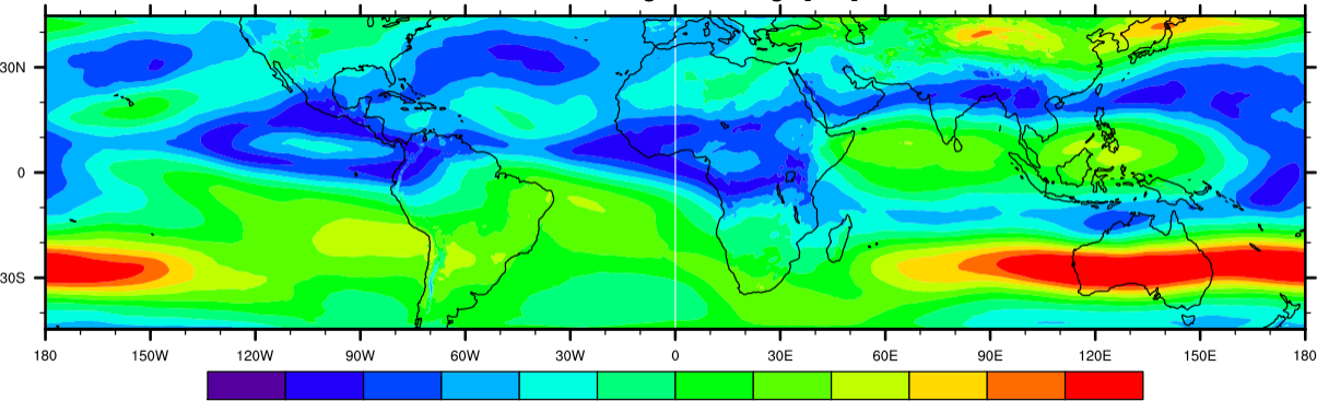
dudz 2004 Aug-Oct average [m/s]
