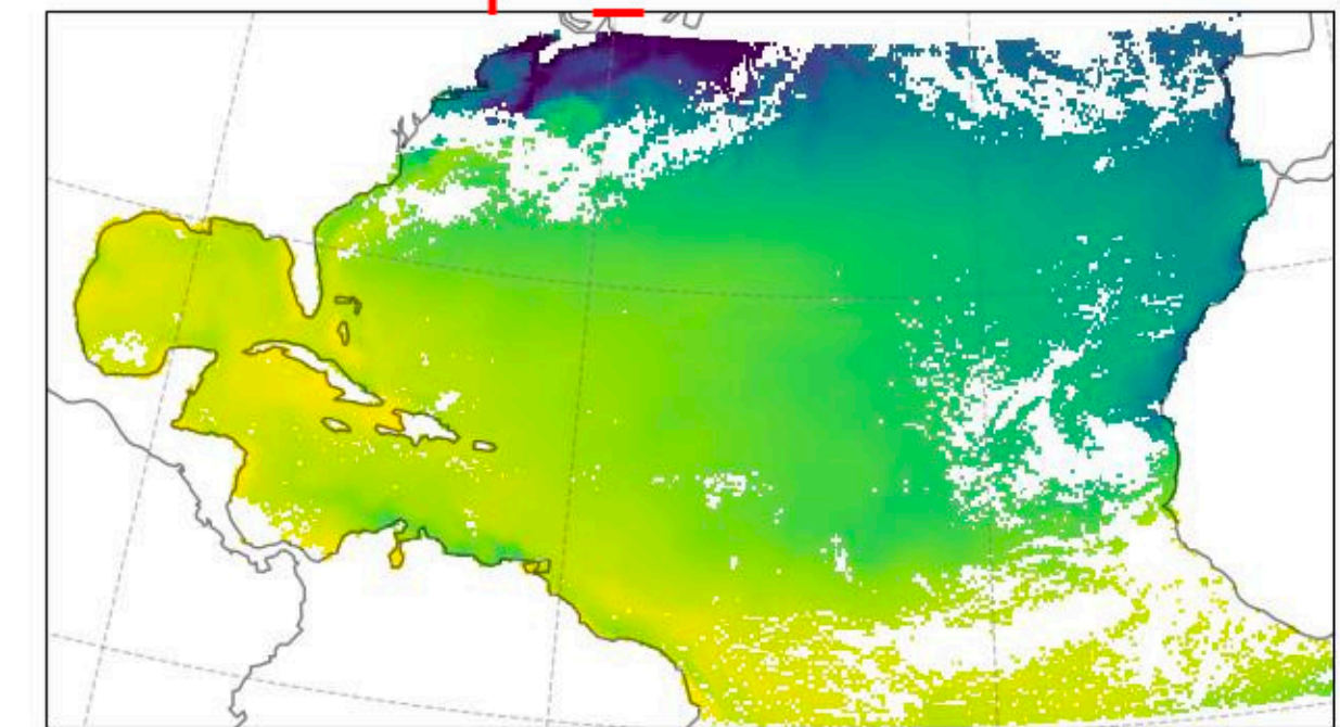
oops_masked
