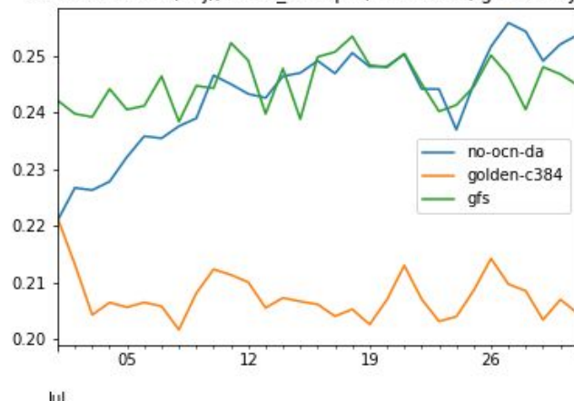
mean abs OmB (adj), avhrr_metop-b, channel 3, global day-bin
