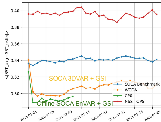
mean abs OmB (adj), avhrr_metop-b, channel 3, global day-bin
