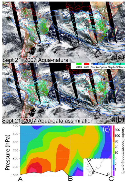
Fig. 4. GOES (red) and MODIS Aqua (green) active fire hotspots and NAAPS 550-nm smoke optical depths overlaid on MODIS Aqua RGB for the South America and Africa transport event of September 21, 2007. Included are optical depths from the (a) natural and (b) optical depth data assimilation runs. (c) Cross section of South American smoke along the center of the plume from Amazonia into the South Atlantic Ocean.
